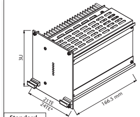
Standard Eurocassette (pluggable module for 19" sub-rack) approx. 1.7 kg *) applicable to 5 V output models
