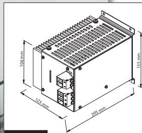
Optional Chassis mount approx. 2.1 kg
