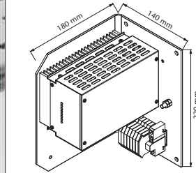
Optional Wall mount approx. 3.2 kg
