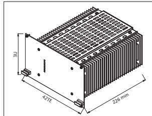
Standard Eurocassette (pluggable module for 19" sub-rack) approx. 4.0 kg
