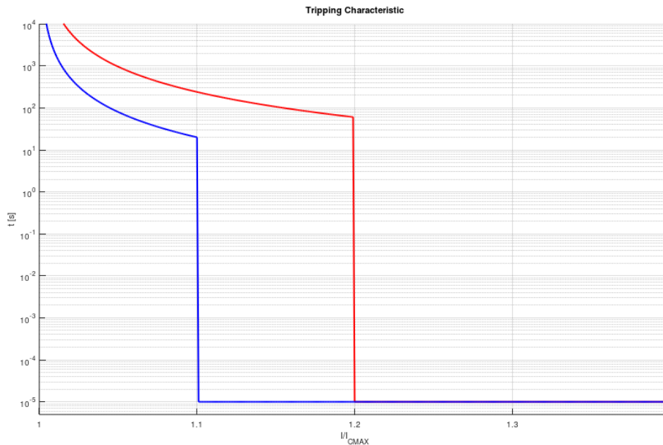
Figure 2 Tripping characteristics
