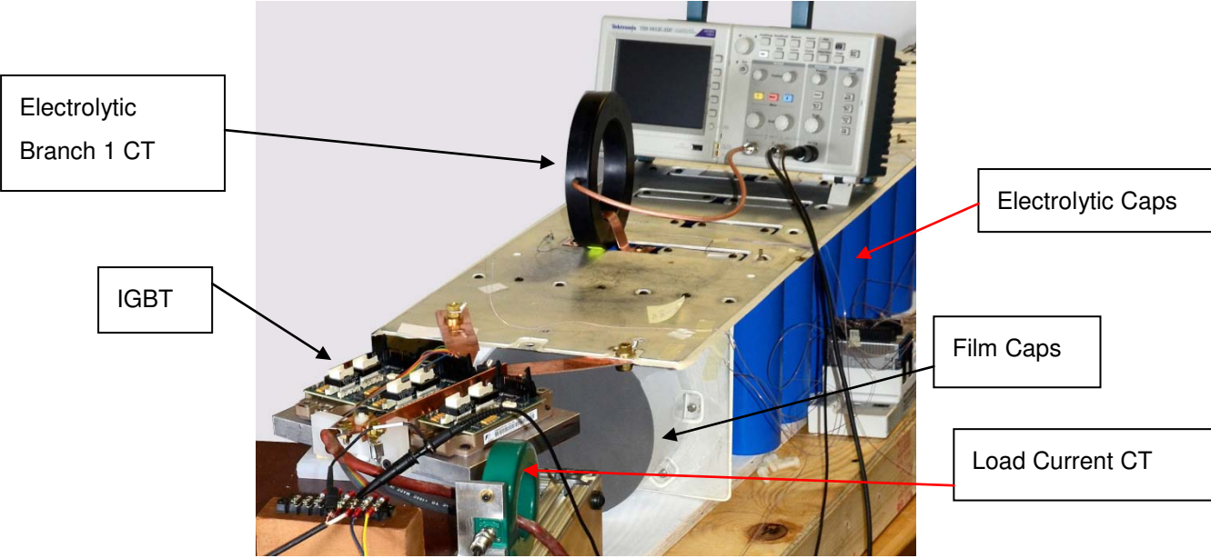
Fig. 6. Photograph of the hybrid DC link capacitor prototype bench testing configuration.
