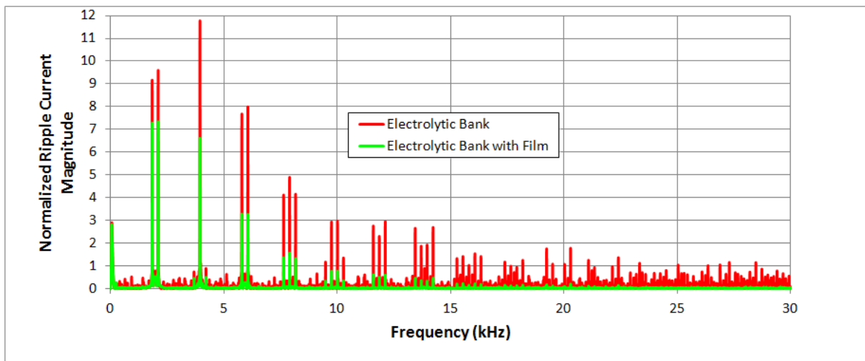
Fig. 2. Illustration of ripple current harmonic reduction by adding a parallel 2mF Power Ring Film Capacitor™ to an existing 40mF electrolytic bank.
