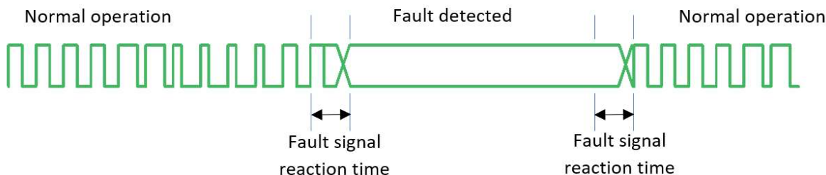
Figure 5: Fault-pin signal illustration
