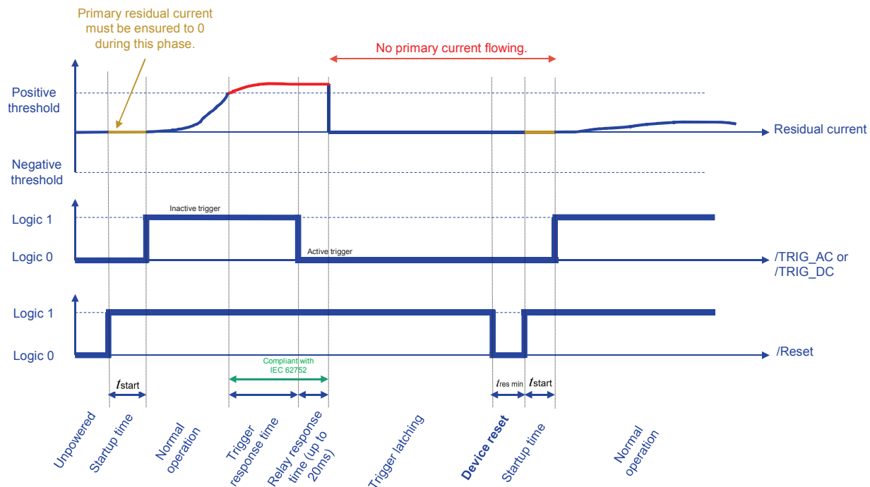
Figure 3: output triggers latching
