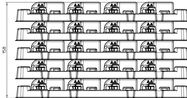
Theoretical stack-up for CDSR 0.07-NPDT
