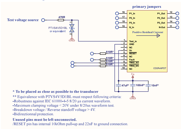
Figure 1: typical mounting and interfacing
