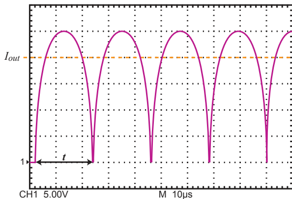
Typical output current waveform.
