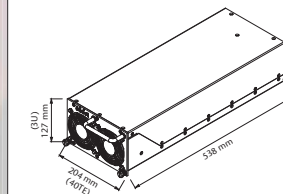
Standard Pluggable module (for 3U sub-rack) approx. 17 kg
