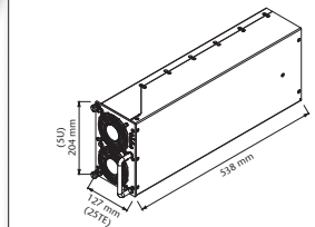
Standard Pluggable module (for 5U sub-rack) approx. 17 kg
